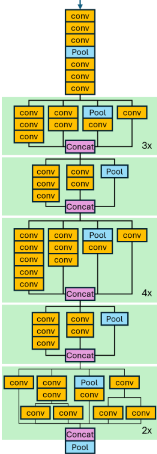
Figure 2. InceptionV3 Architecture
