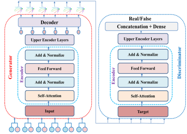
Figure 3. An overview of the proposed model.
