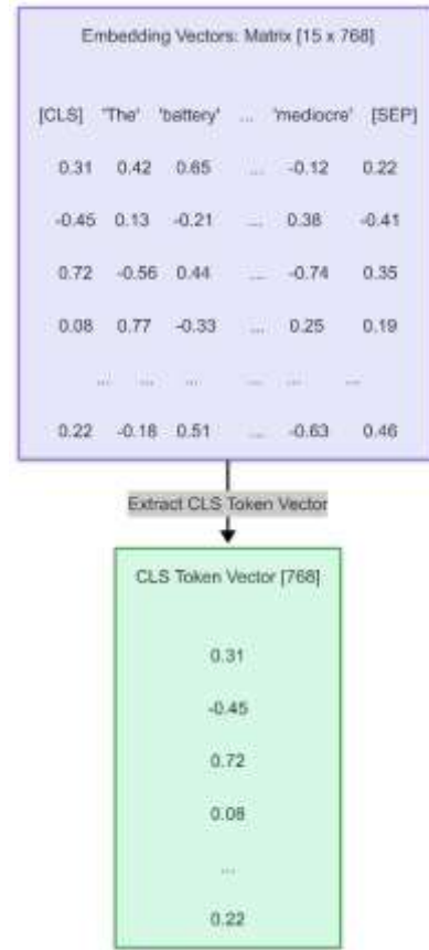
Figure 3. Extract CLS Token From Global Context Features.
