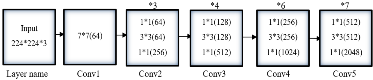
Figure 3. Block diagram of ResNet50 architecture.
