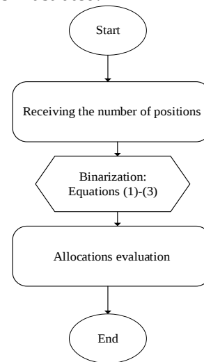
Figure 3. Formulation of allocation problem in Cheetah Algorithm.
