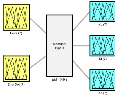
Figure 4. The fundamental design of a fuzzy controller for managing angles and z –position.
