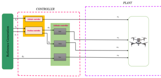
Figure 2. Control architecture.
