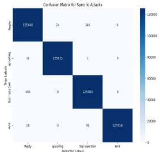
Figure 7. Confusion matrix.
