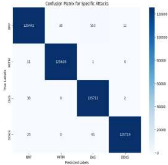
Figure 5. Confusion matrix.
