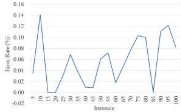
Figure 3. Error percentage of results obtained by DSA algorithm in comparison with CPLEX
