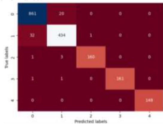
Figure 8. Confusion matrix of the proposed method on the Defungi dataset.
