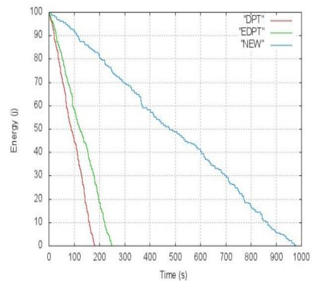
Figure 6. Residual energy of nodes when target speed is 1m/s.
