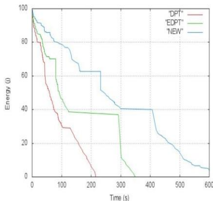
Figure 5. Residual energy of nodes when target speed is 5m/s.
