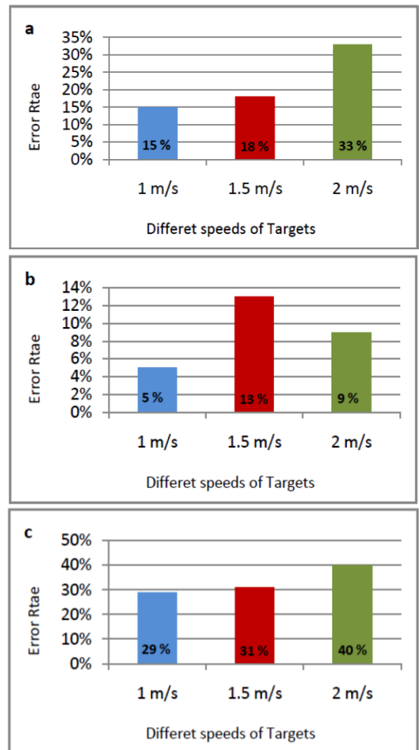
Figure 7. Error rate with respect to different speeds of target. a) DPT, b) EDPT, and c) (TTBBVG) proposed protocol.
