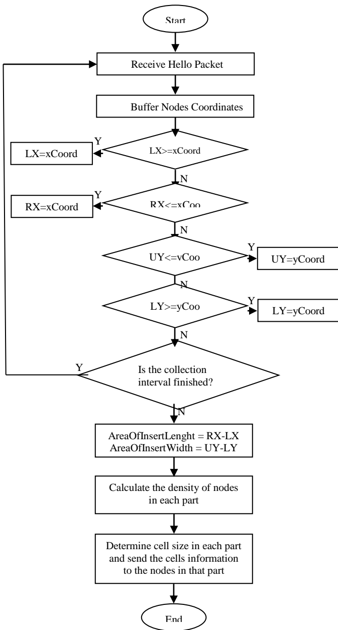
Figure 3. Calculation of length and width of area of interest and cells using sink node.
